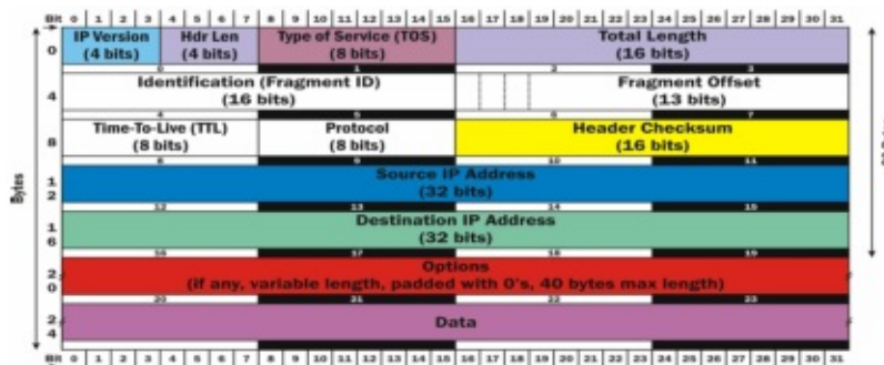
Figure 3.3-b: IPv4 Packet Header
