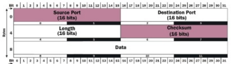
Figure 3.5-a: UDP Packet Header
