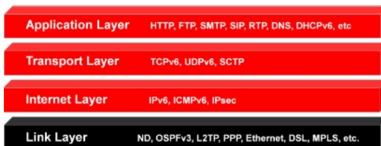
Figure 5.3-a: Four Layer TCP/IPv6 Model
