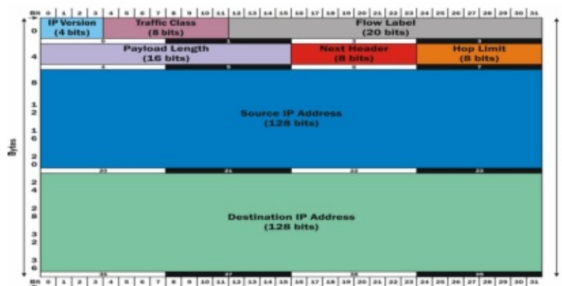
Figure 5.3-b: IPv6 Packet Header
