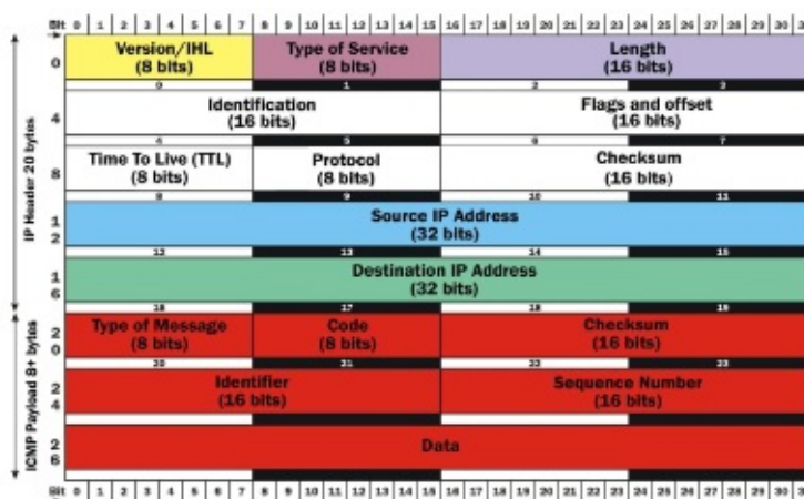
Figure 3.3-c: ICMPv4 Message Syntax
