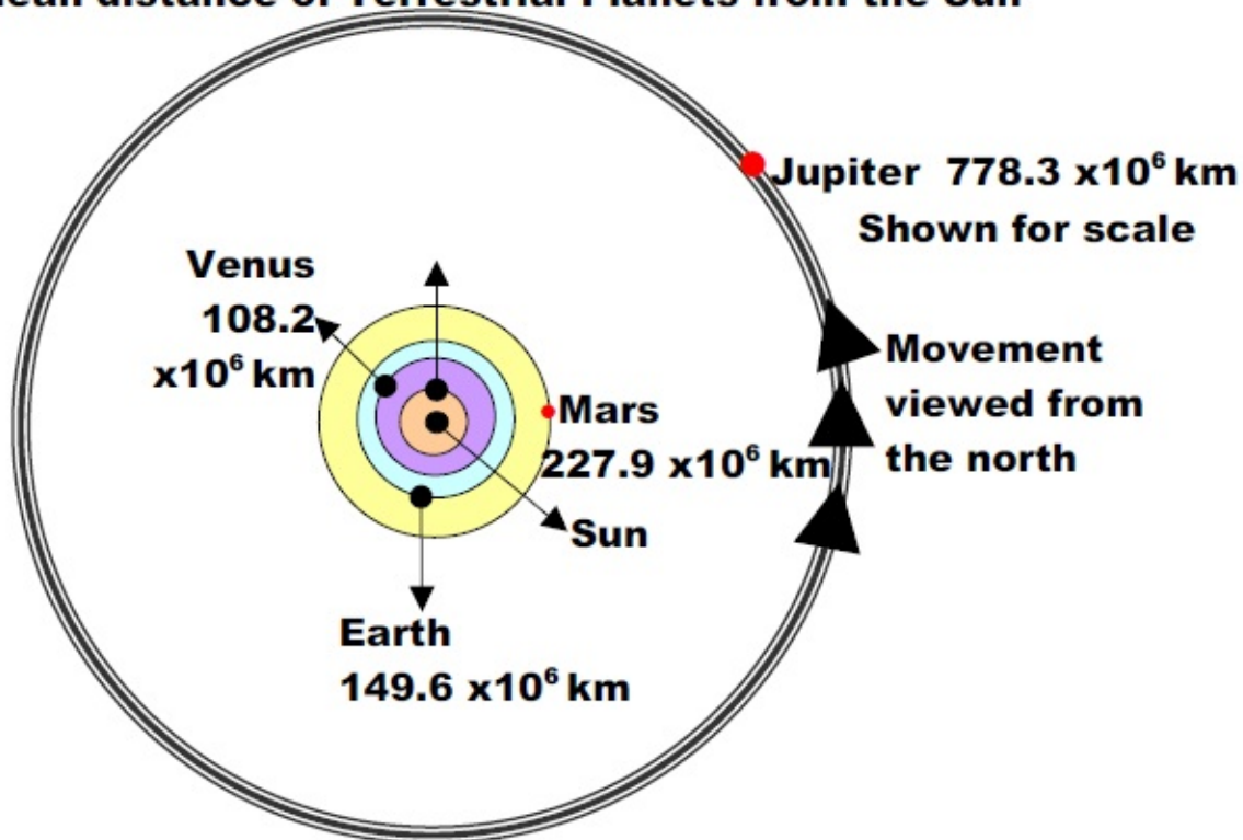
Mean distance of Terrestrial Planets from the Sun
