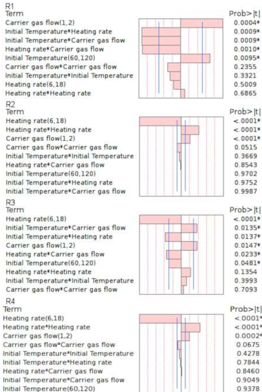
Figure 3. Significance charts of the factors for the different responses.
