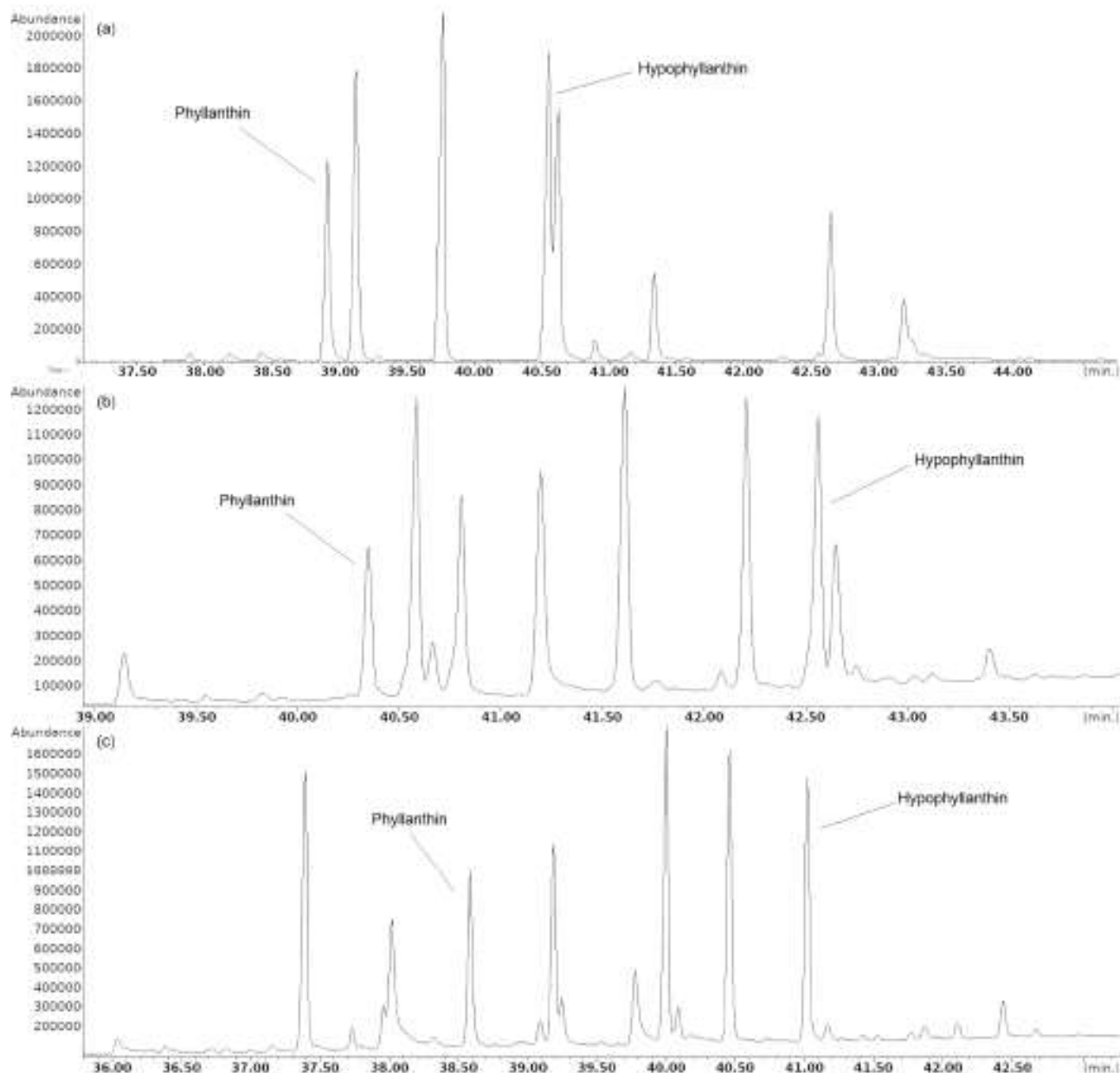
Figure 2. Total ion chromatograms of P. niruri in different columns (a) DB-5ms (b) DB-35 and (c) DB-17HT in the same method.
