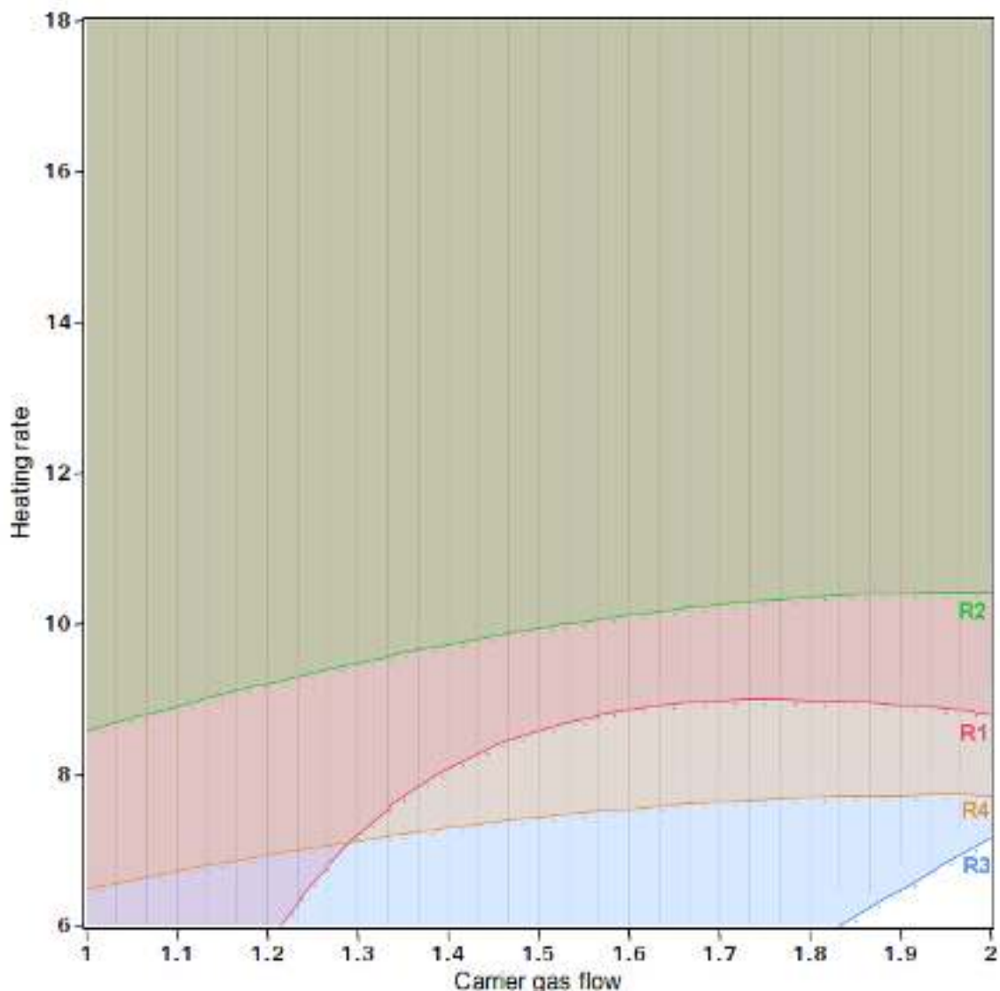
Figure 4. Contour chart of the four responses.
