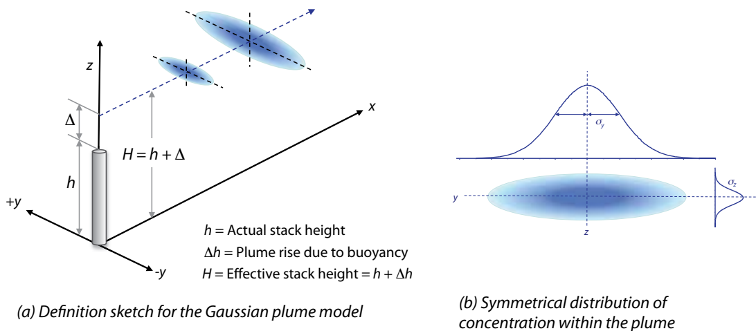
Figure 7.4 Ideal Gaussian plume dispersion. (a) Dispersion of a plume released under stable conditions at an effective height H . The pollutant disperses laterally and vertically as the plume moves downwind. (b) A view of the plume looking down the centerline shows the peak concentration is at the centerline and the the bell-shaped (Gaussian) distributions of concentration.
