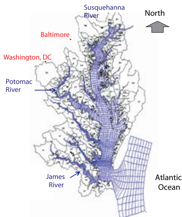
Figure 8.17 Structure of a water quality model for Chesapeake Bay, one of the most important estuaries in the United States (U.S. EPA 2010).
