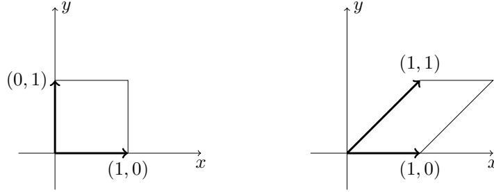
Figure 12.4: SL_2(\mathbb{R}) acting on the unit square
