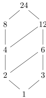
Figure 19.7: A partial order on the divisors of 24
