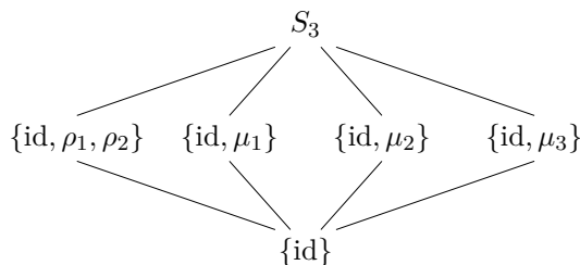
Figure 4.8: Subgroups of S_3
