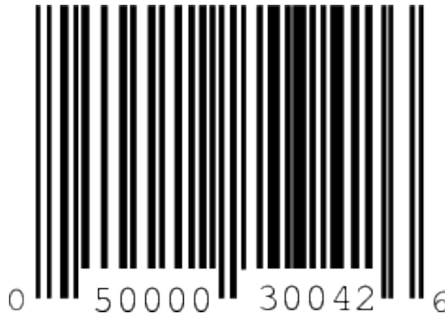
Figure 3.32: A UPC code
