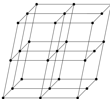
Figure 12.17: A crystal structure in \mathbb{R}^3
