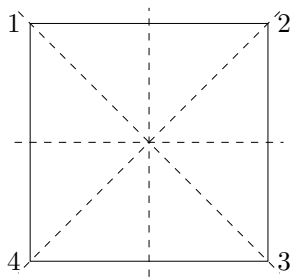
Figure 5.25: The group D_4
