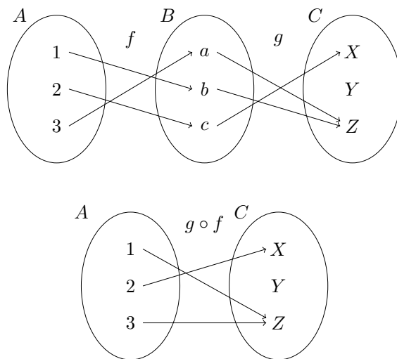
Figure 1.9: Composition of maps
