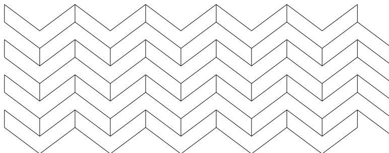
Figure 12.16: A wallpaper pattern in \mathbb{R}^2
