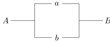
Figure 19.26: a \vee b
