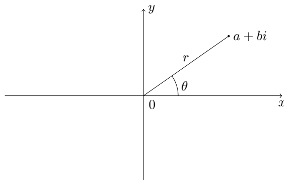
Figure 4.18: Polar coordinates of a complex number
