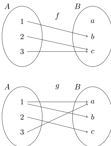
Figure 1.6: Mappings and relations
