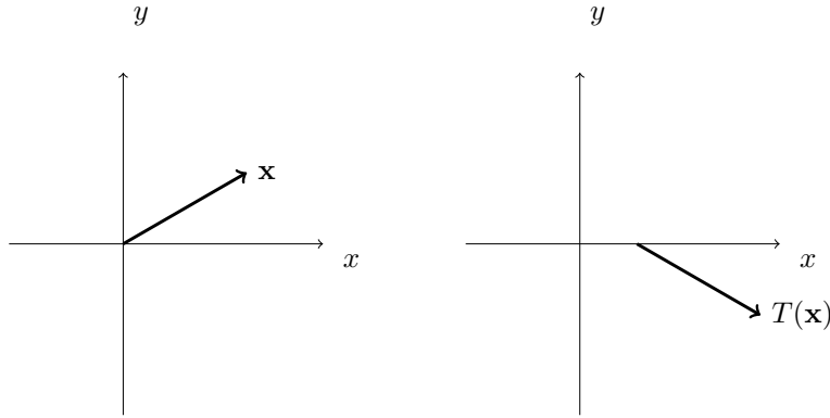
Figure 12.12: Glide reflections
