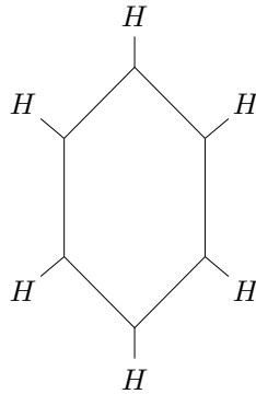
Figure 14.28: A benzene ring
