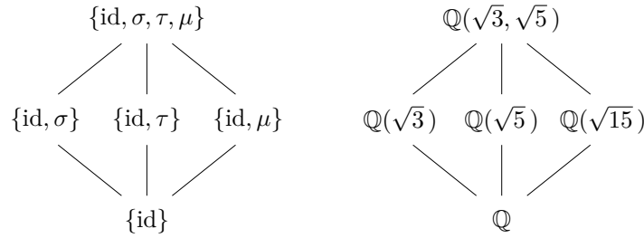
Figure 23.21: G(\mathbb{Q}(\sqrt{3}, \sqrt{5})/\mathbb{Q})
