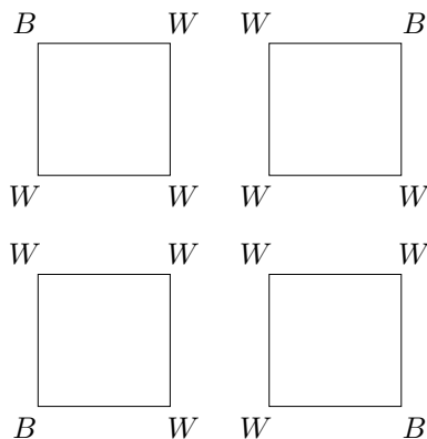
Figure 14.17: Equivalent colorings of square
