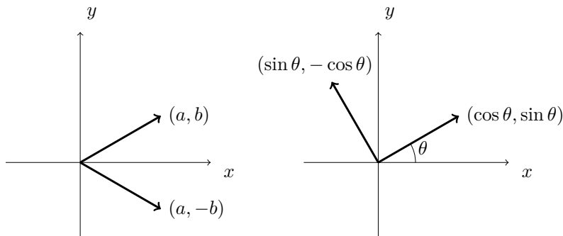
Figure 12.9: O(2) acting on \mathbb{R}^2
