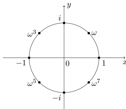
Figure 4.27: 8th roots of unity
