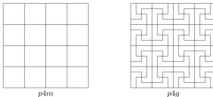
Figure 12.24: The wallpaper groups p4m and p4g
