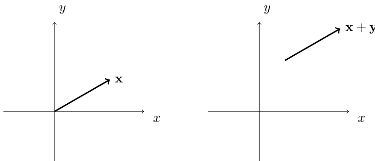
Figure 12.11: Translations in \mathbb{R}^2
