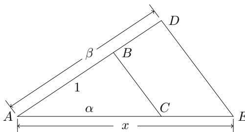
Figure 21.36: Construction of products
