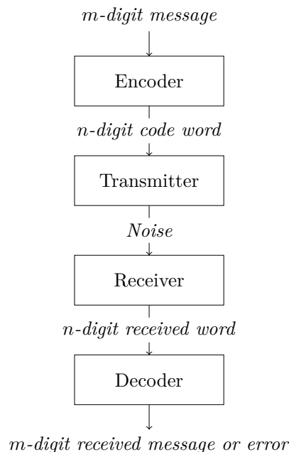
Figure 8.1: Encoding and decoding messages
