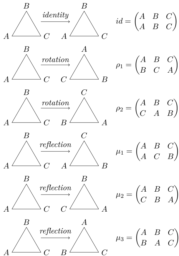
Figure 3.6: Symmetries of a triangle
