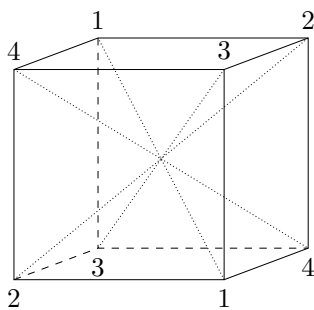
Figure 5.26: The motion group of a cube
