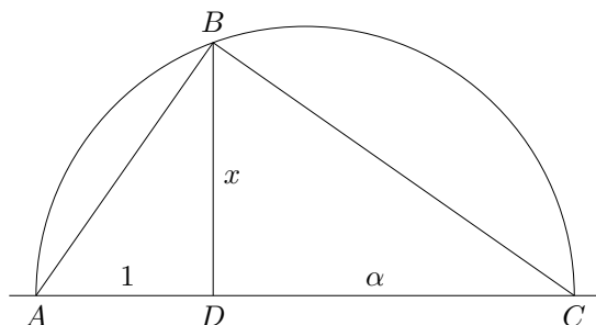
Figure 21.38: Construction of roots
