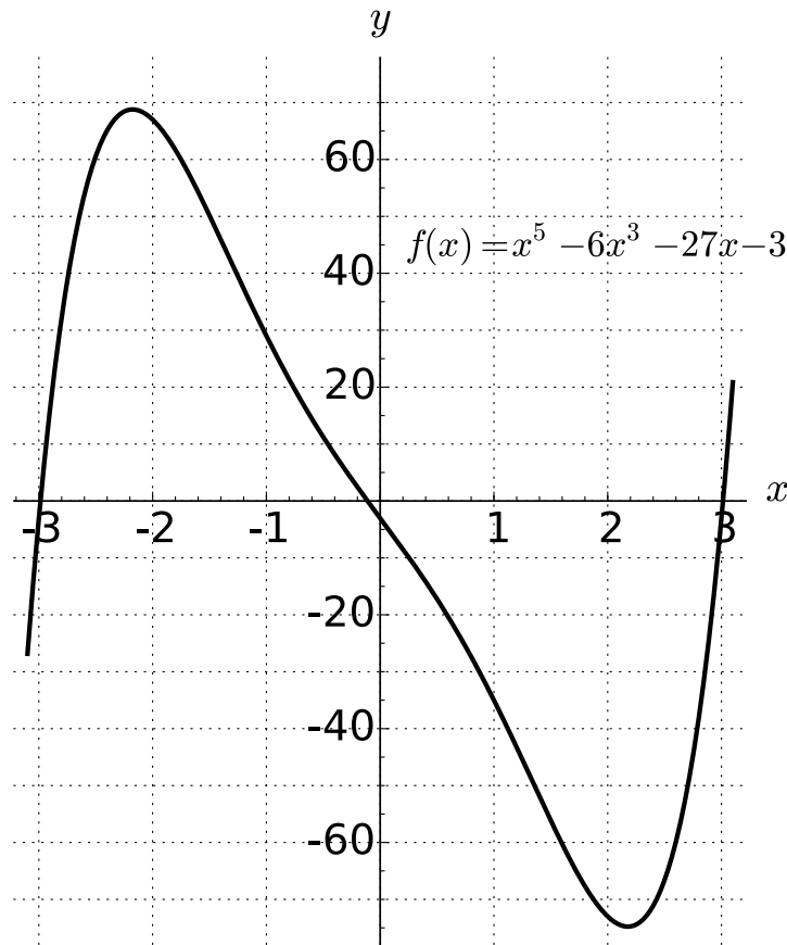
Figure 23.31: The graph of f(x) = x^5 - 6x^3 - 27x - 3
