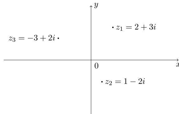
Figure 4.17: Rectangular coordinates of a complex number
