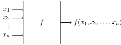
Figure 14.24: A switching function of n variables
